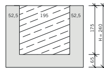
B = 300 mm
