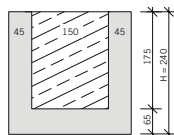
B = 240 mm
