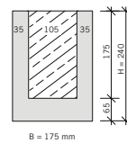
B = 175 mm
